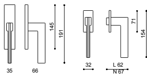
C228S - fixed window slider
