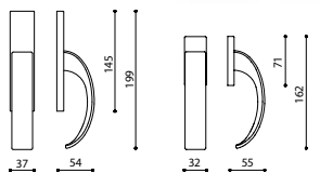
C225S - fixed window slider
