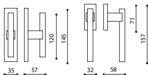
C204S - fixed window slider
