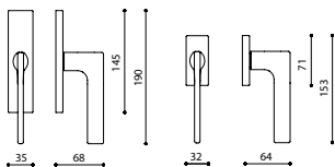
C238S - fixed window slider
