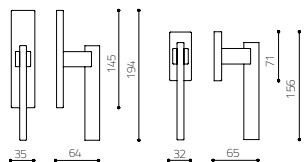
C205S - fixed window slider
