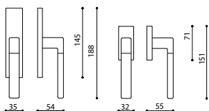
C195S - fixed window slider
