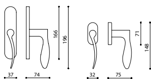
C116R - fixed window slider
