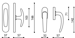
C103R - fixed window slider
