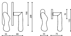
C232R - fixed window slider
