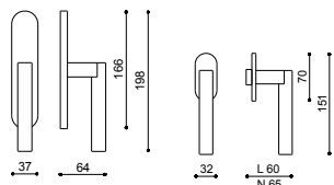
C229R - fixed window slider
