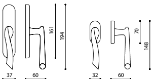
C173R - fixed window slider
