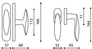
C175R - fixed window slider
