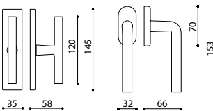
C128R - fixed window slider
