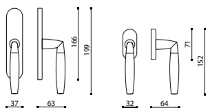
C186R - fixed window slider
