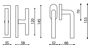
C130R - fixed window slider
