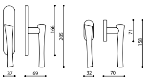
C154R - fixed window slider
