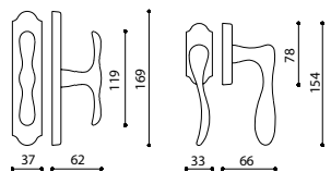
C169R - fixed window slider
