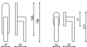
C195R - fixed window slider
