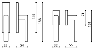
C195S - fixed window slider
