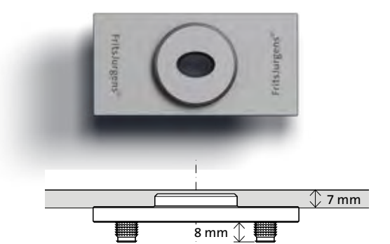
Floor plate Flush squared – Non-adjustable
