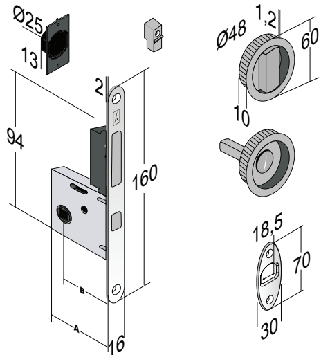
Single Face Plate with Integrated Finder Pull.
