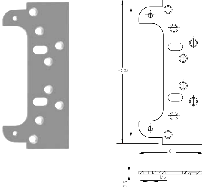
Offset Fixing Plate Dimensions
